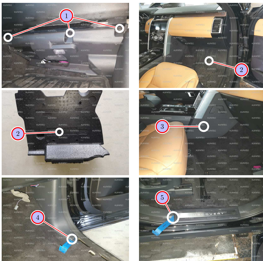
Figure 4: Removing trim panels passenger's side
