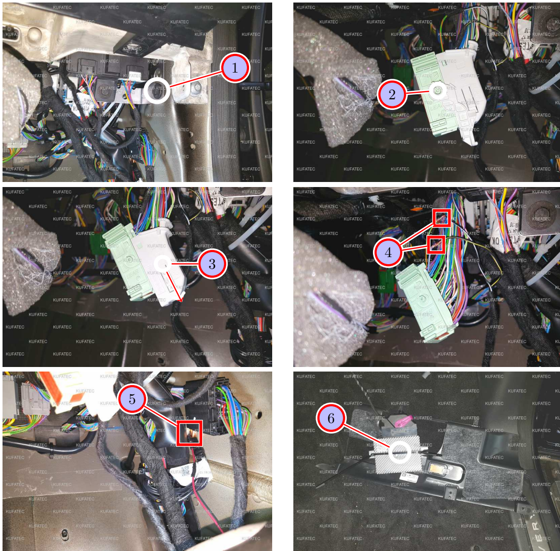
Figure 7: Connection cable set
