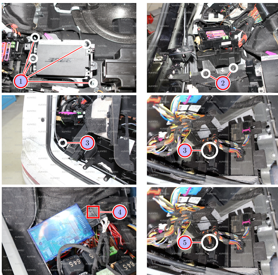
Figure 6: Removing fuse box in the hatch / Connection Sound Booster
