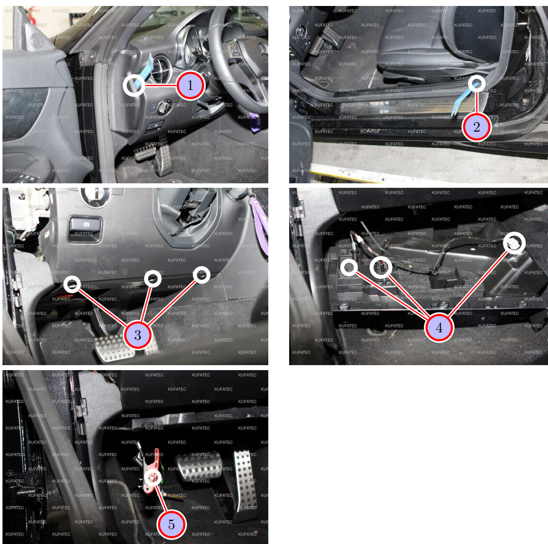
Figure 4: Removing trim panel of the dashboard
