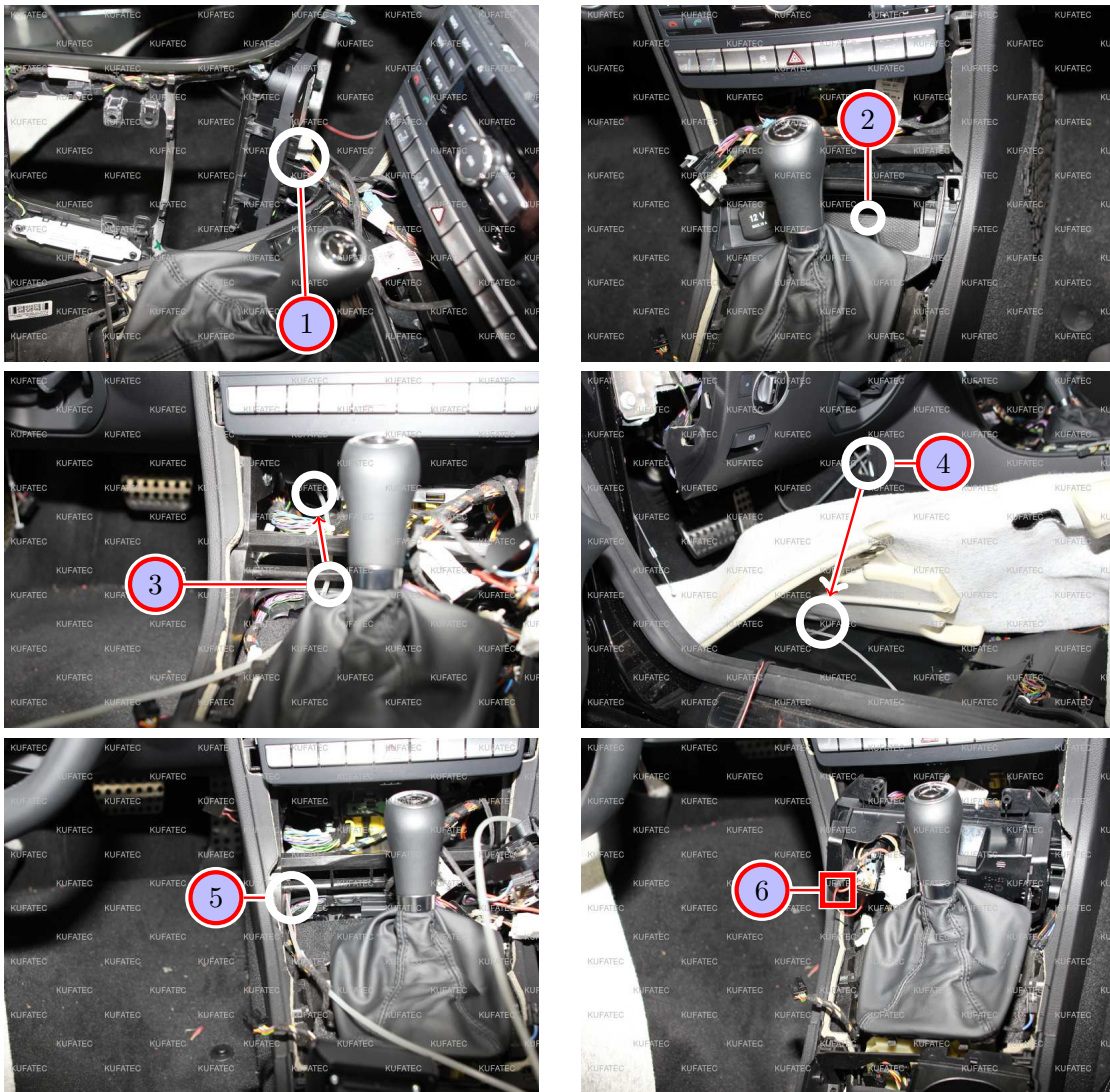
Figure 9: Connection ignition lead
