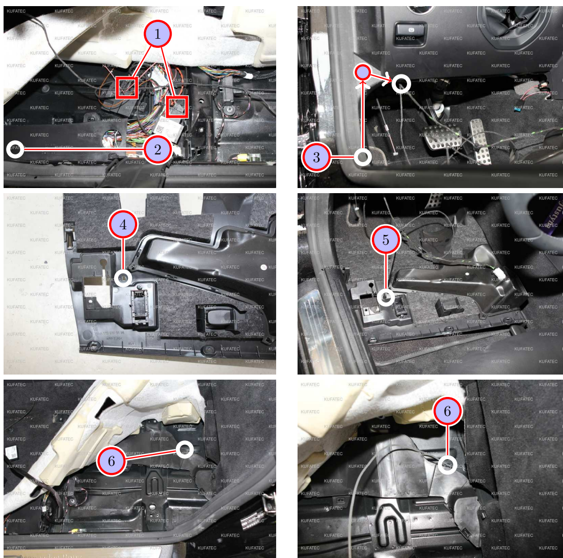
Figure 10: Installation pushbutton / routing connecting cable sound generator
