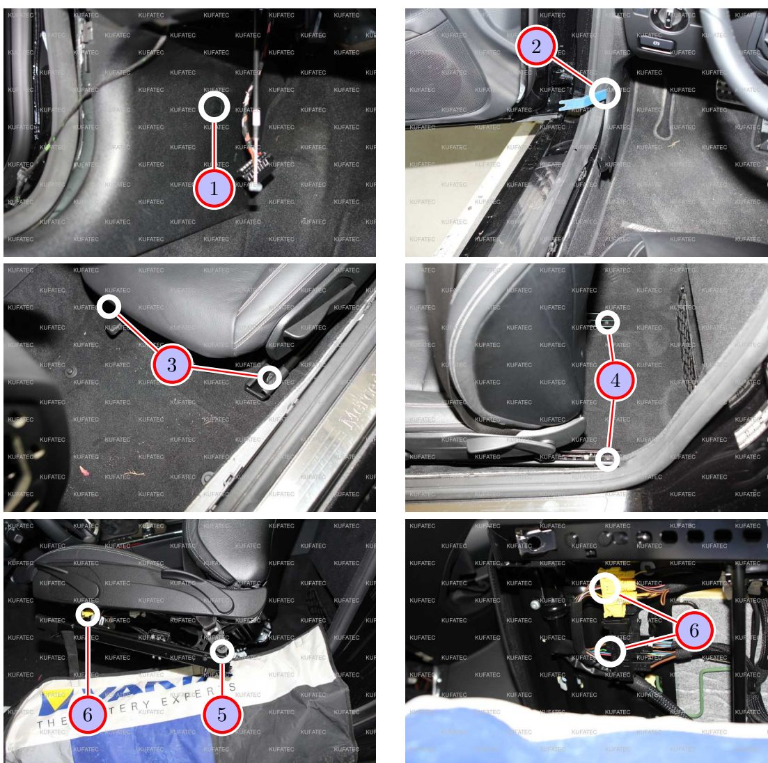
Figure 5: Removing driver's seat
