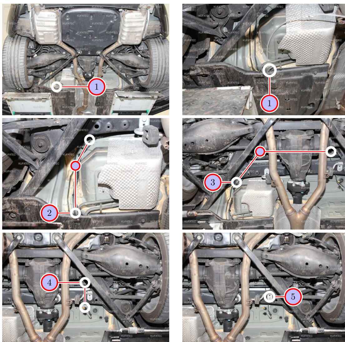
Figure 11: Routing connecting cable sound generator
