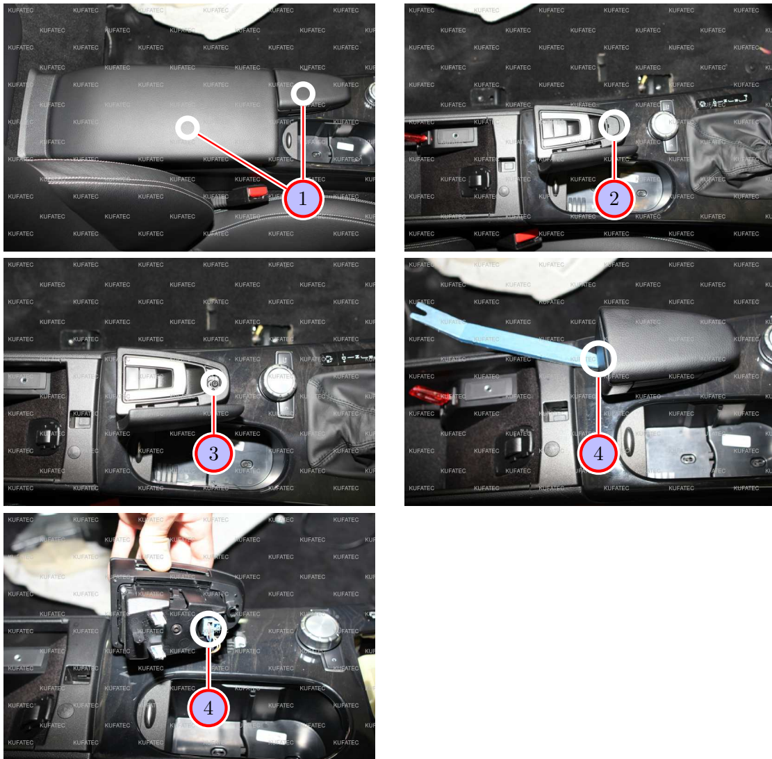
Figure 7: Removing center console
