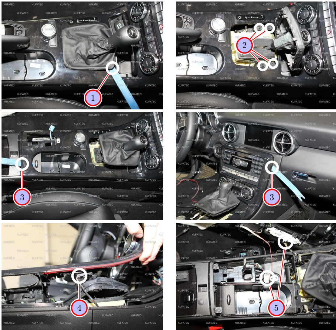
Figure 8: Removing center console
