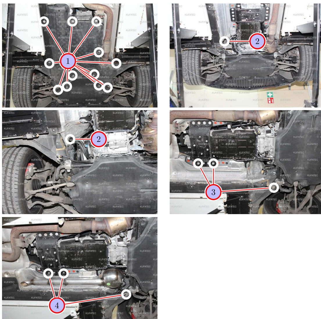
Figure 9: Installation sound generator
