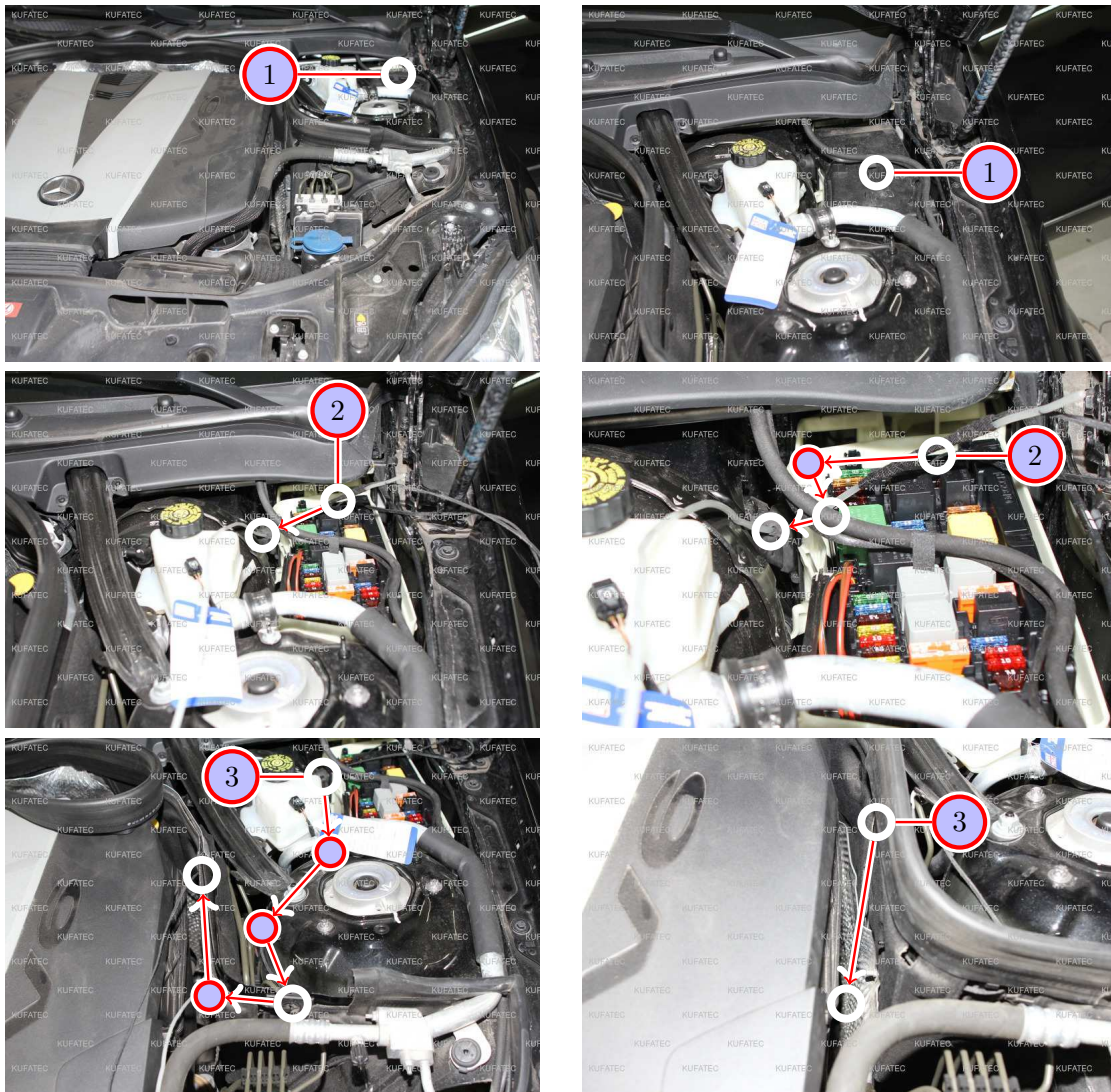
Figure 8: Routing connecting cable of the sound generator
