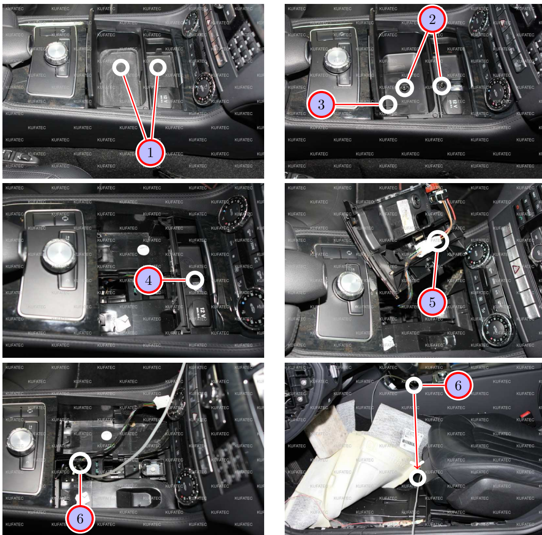
Figure 6: Connection ignition lead
