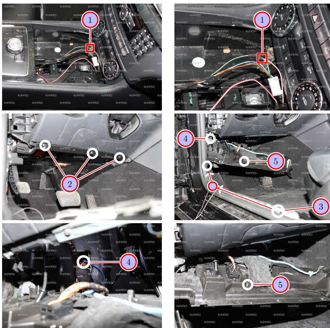
Figure 7: Connection ignition lead / installation pushbutton
