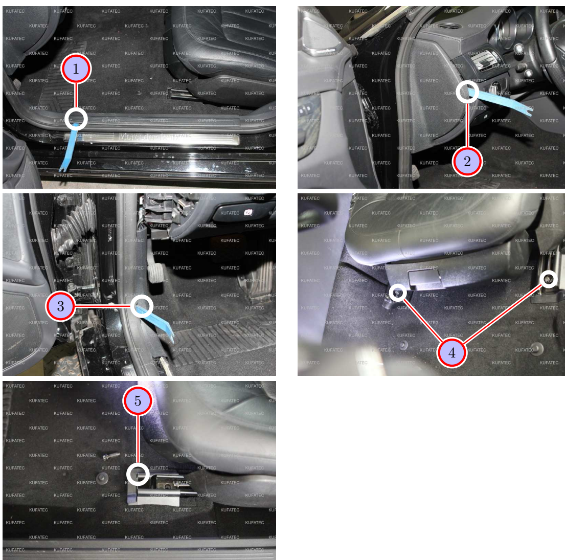
Figure 4: Removing interior trim panel
