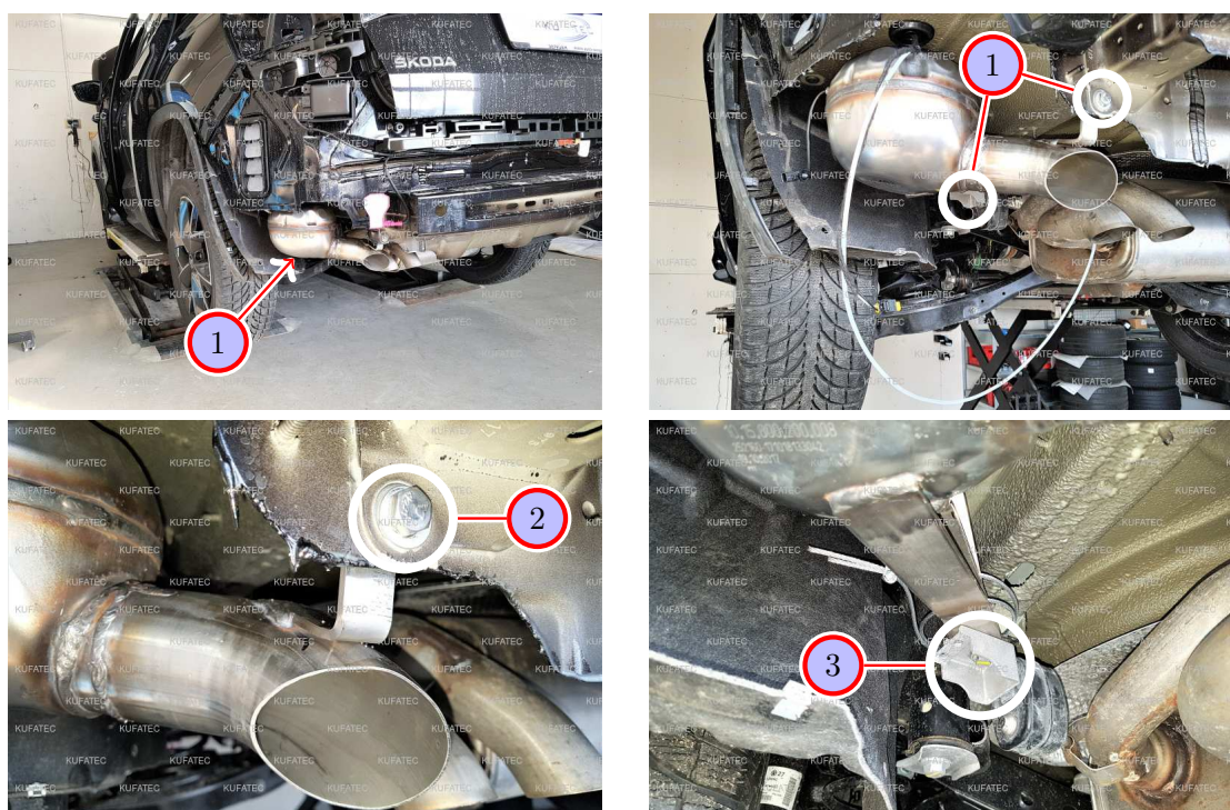
Figure 8: Assembly sound generator
