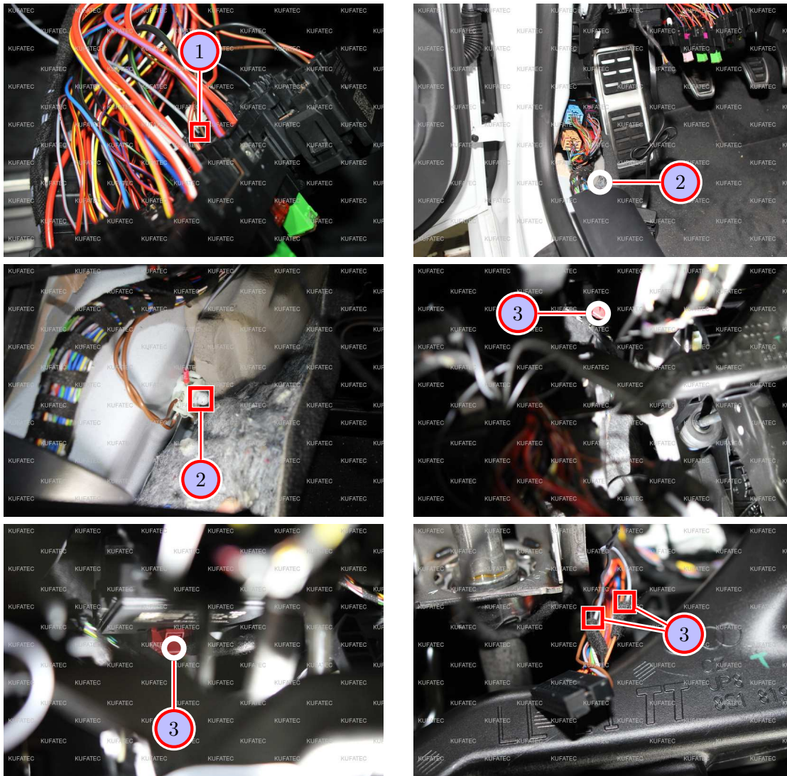
Figure 6: Connection ignition lead / ground / CAN High & CAN Low
