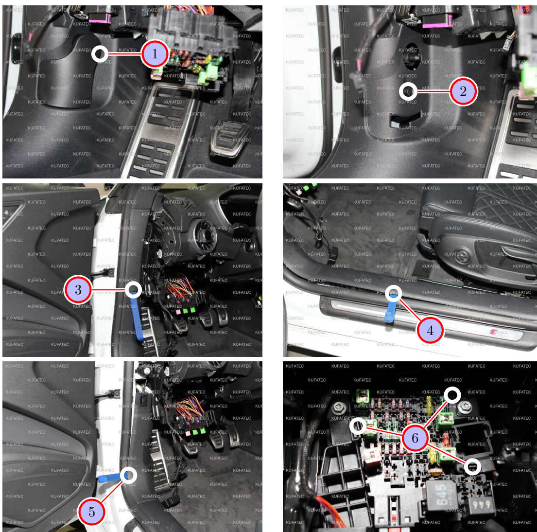
Figure 5: Removing trim panel driver's side front
