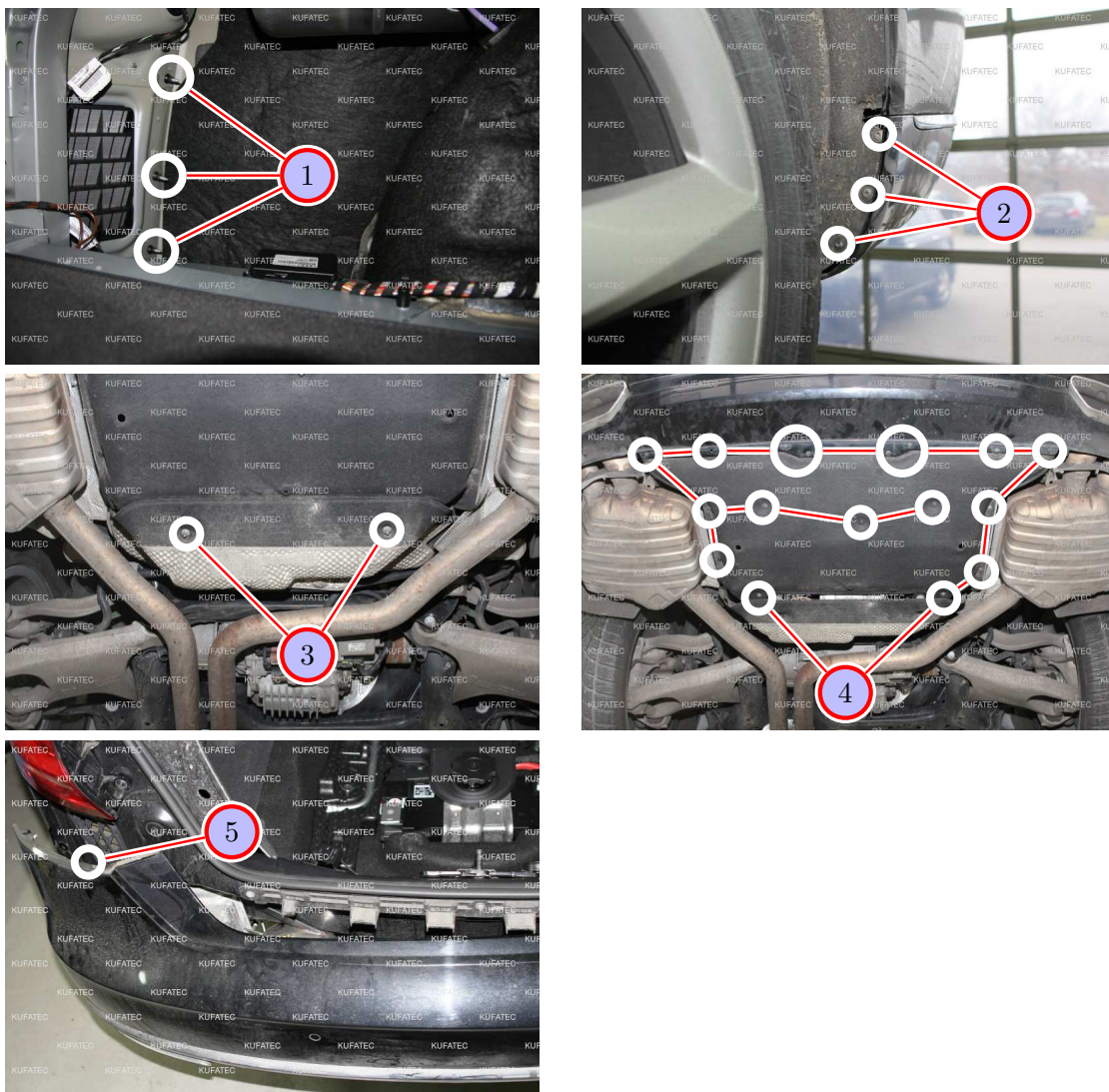
Figure 11: Removing bumper
