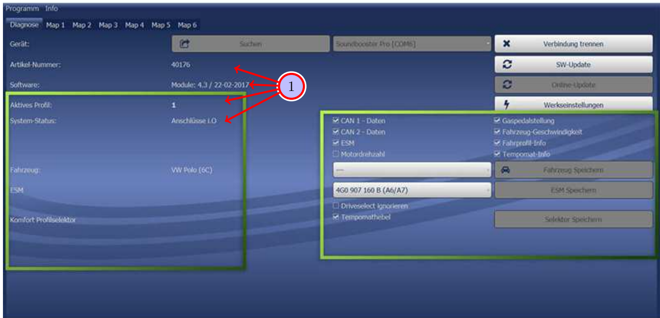
Figure 14: Software
