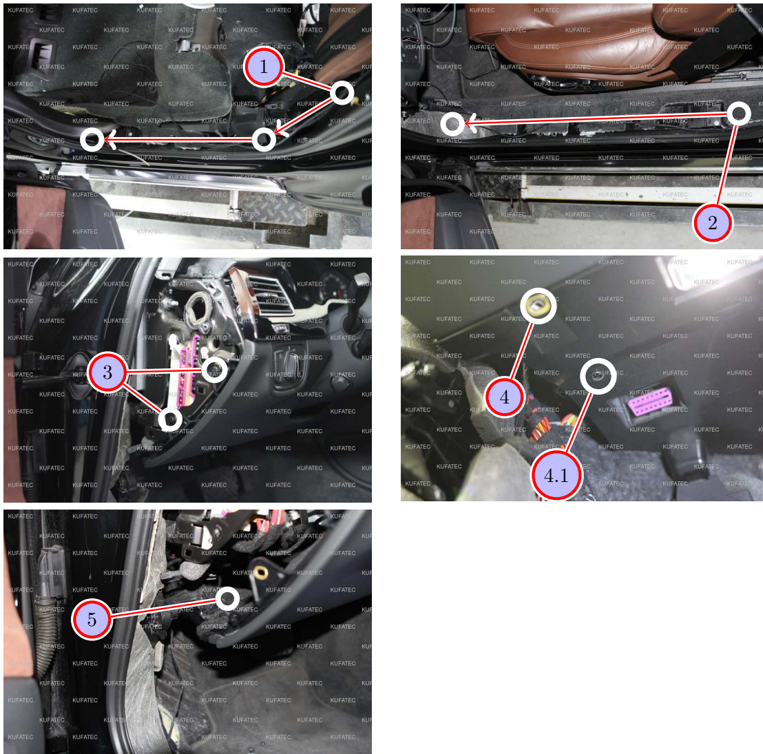
Figure 8: Installation pushbutton
