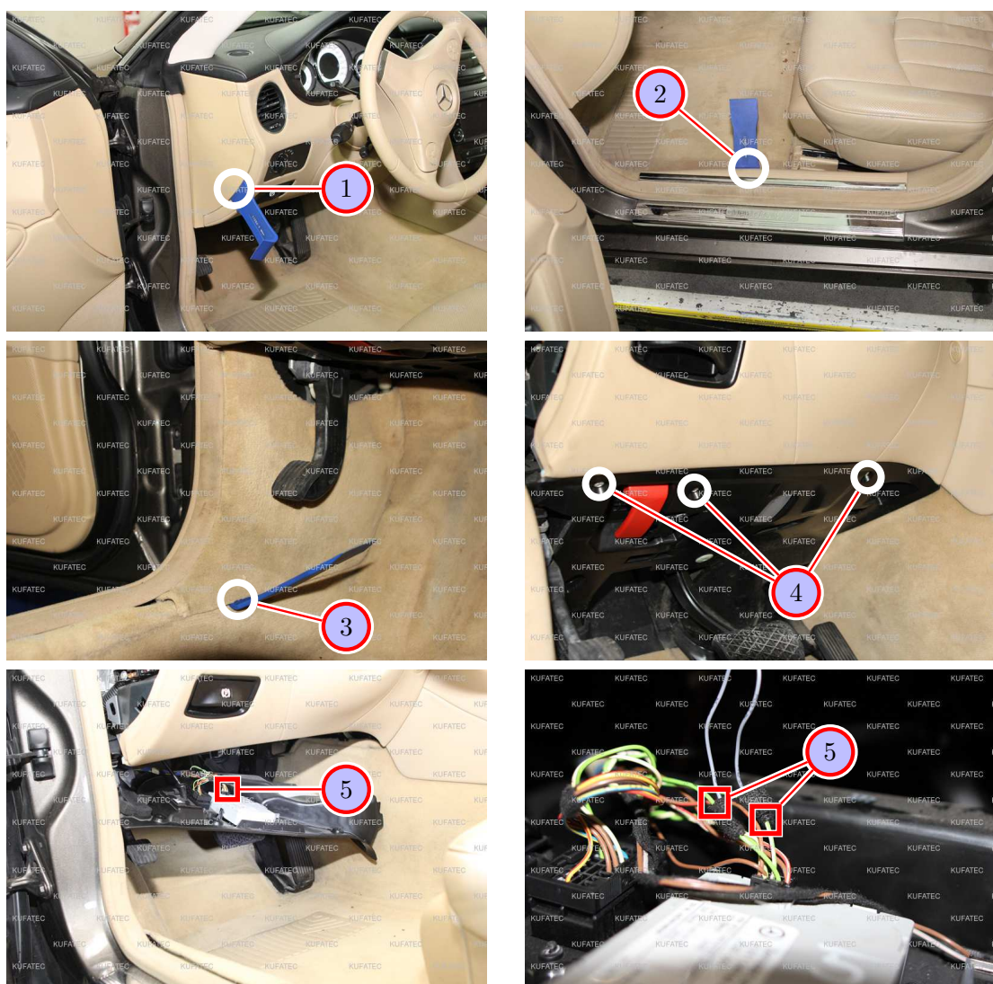
Figure 4: Removing trim panel driver's side / connection CAN High & Low
