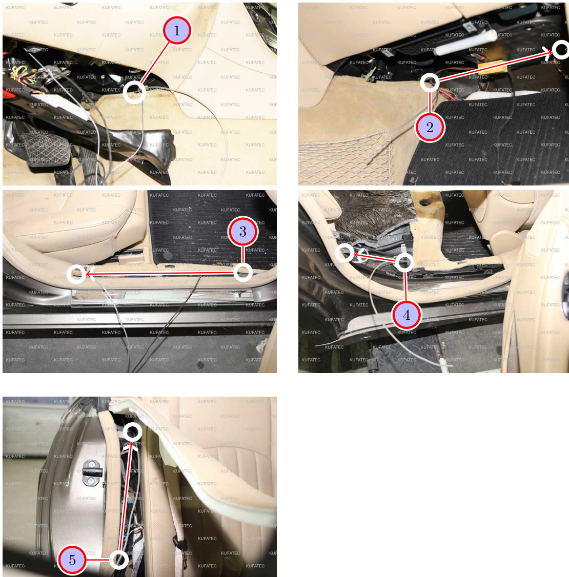
Figure 10: Cable routing to the trunk
