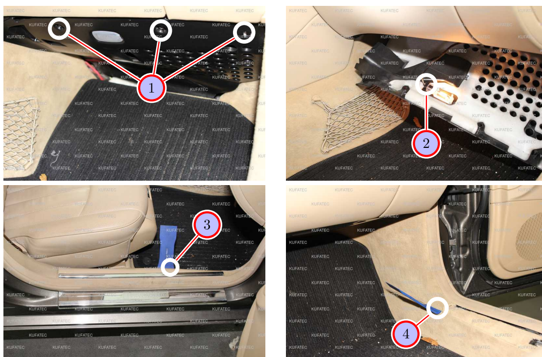
Figure 8: Removing front trim panel passenger's side
