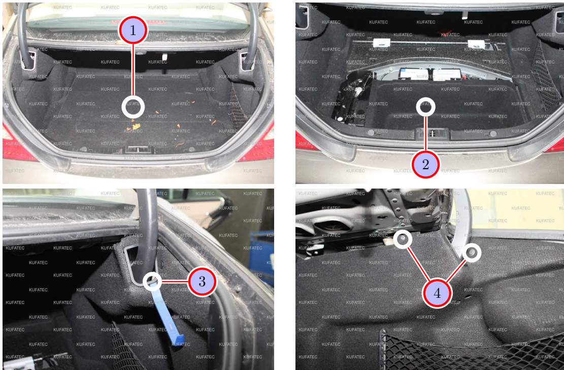
Figure 11: Removing trim panel trunk
