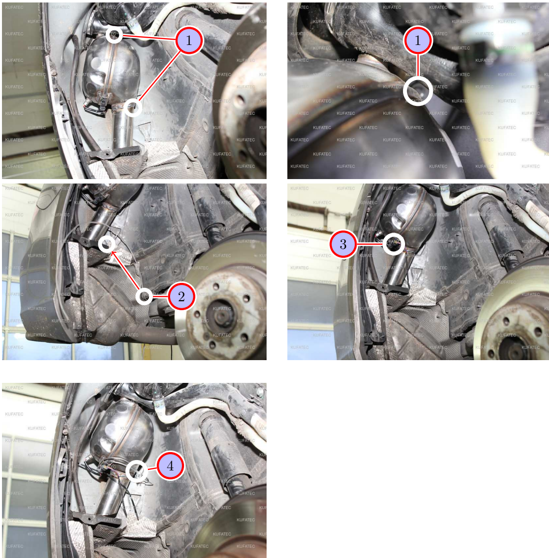
Figure 14: Installation sound generator
