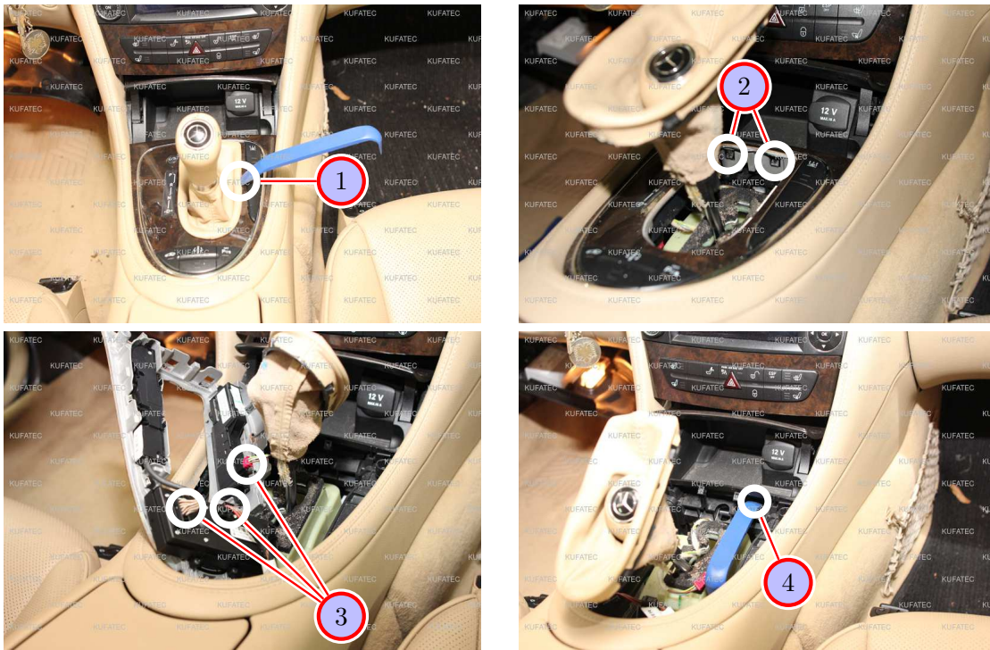
Figure 5: Removing trim panel center console
