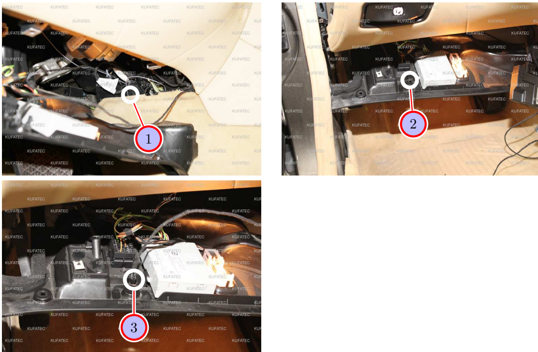
Figure 7: Installation pushbutton / placing control unit & module
