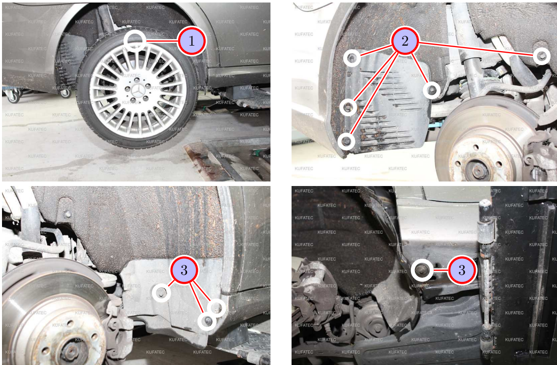
Figure 13: Removing rear interior trim of the wheel housing passenger's side
