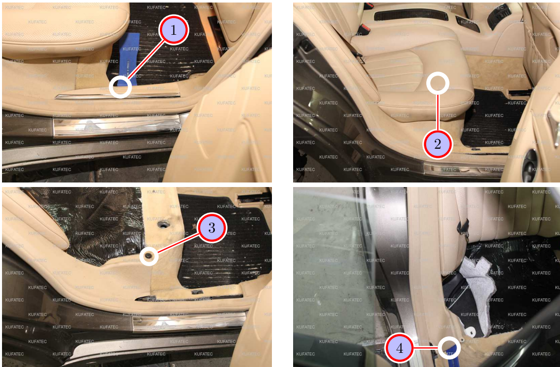
Figure 9: Removing rear trim panel passenger's side
