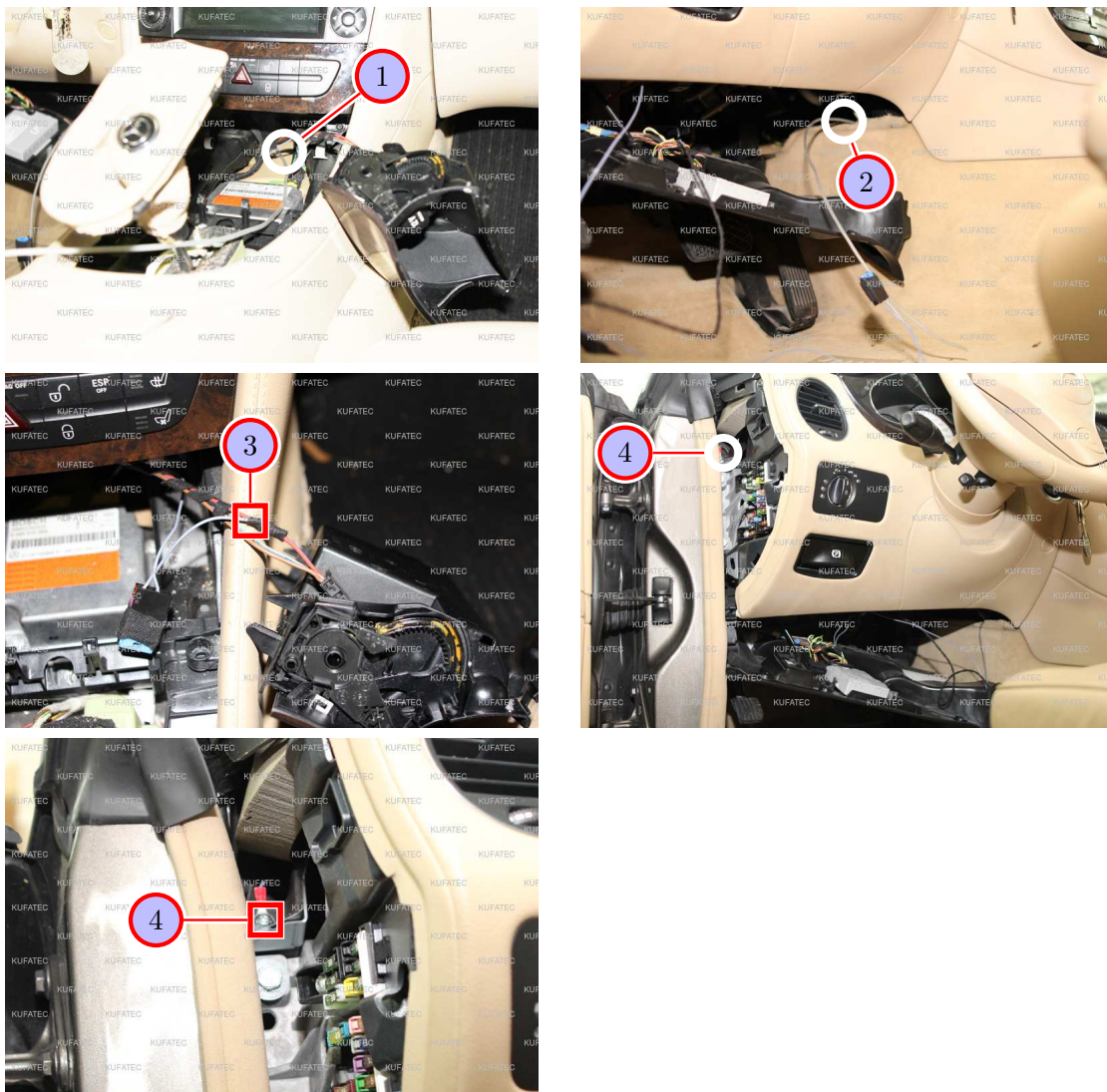
Figure 6: Connection ignition lead / ground
