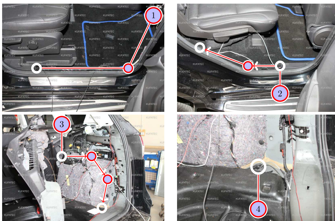
Figure 8: Routing connecting cable sound generator
