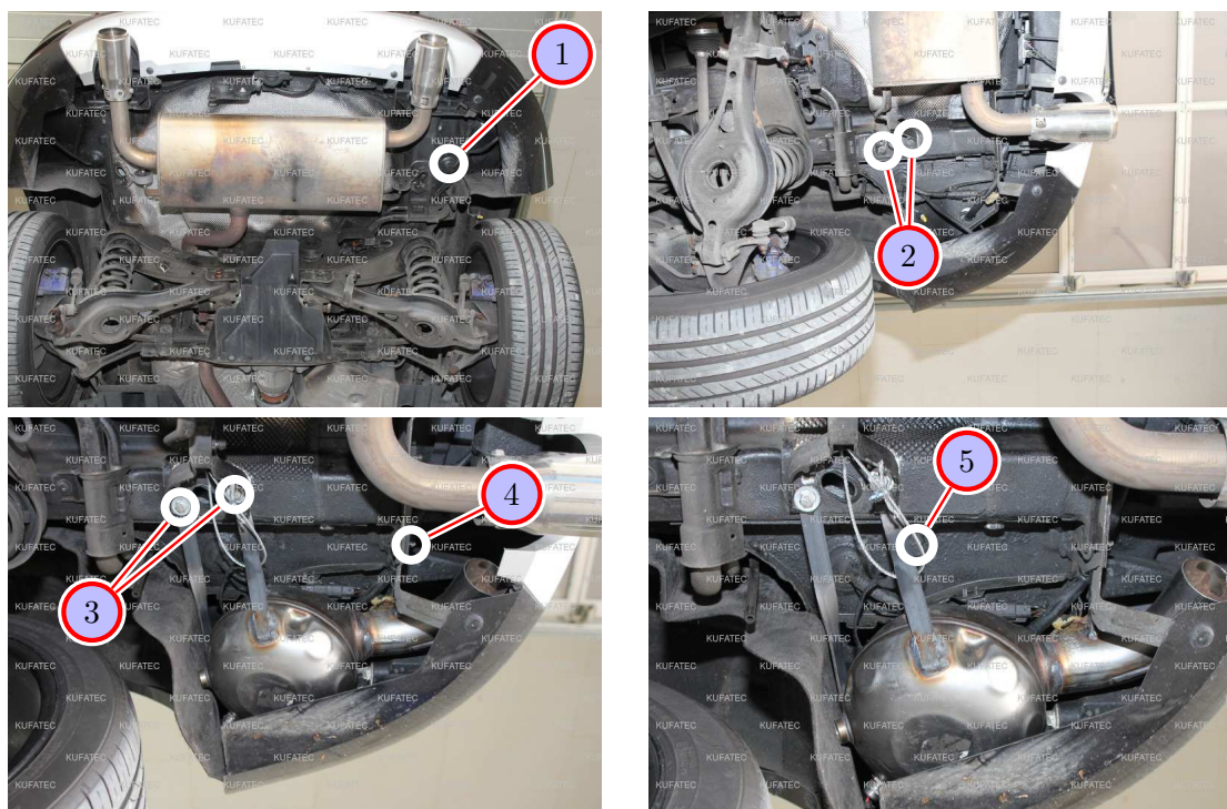
Figure 9: Installation sound generator
