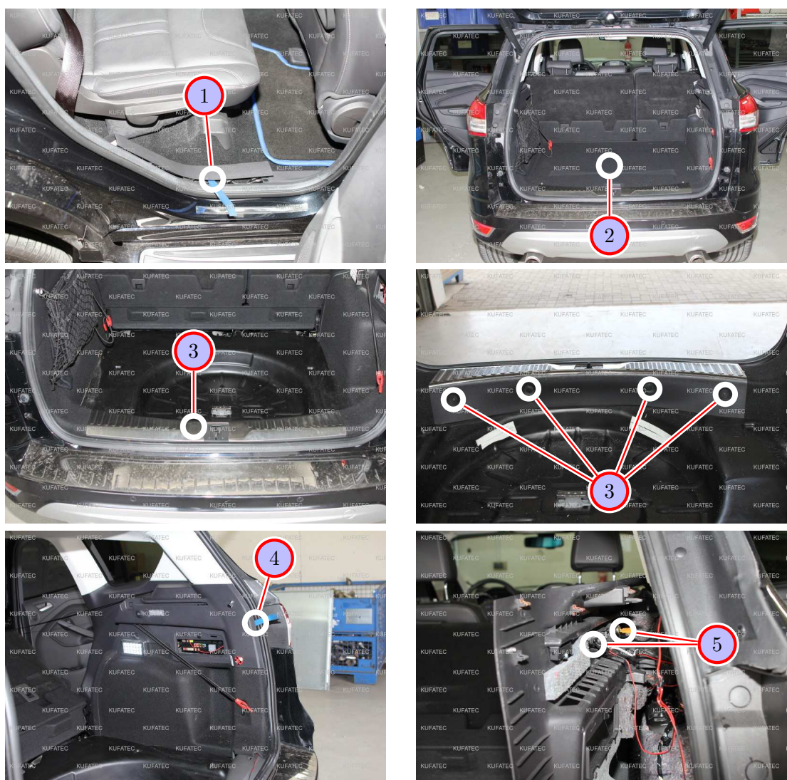
Figure 7: Removing side trim panel trunk
