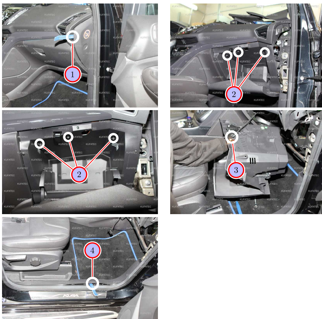
Figure 4: Removing glove compartment
