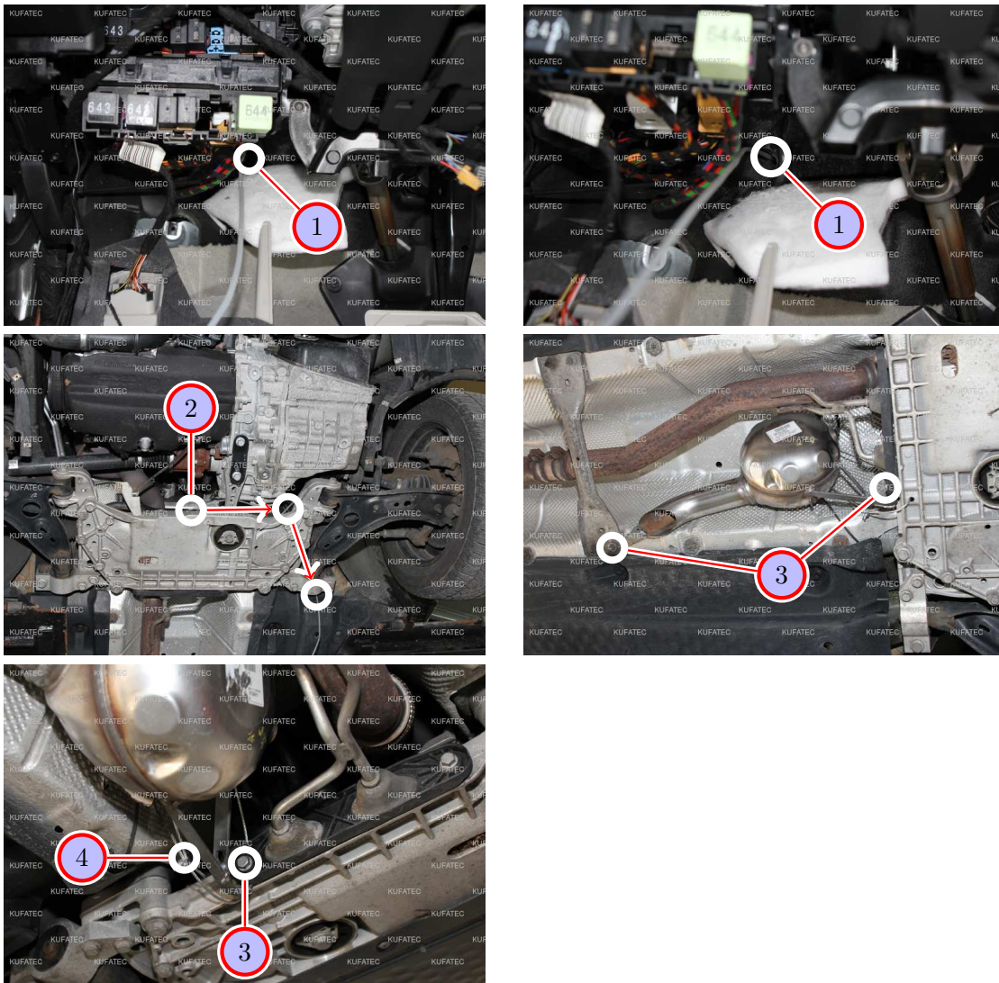
Figure 6: Cable routing and installation sound generator
