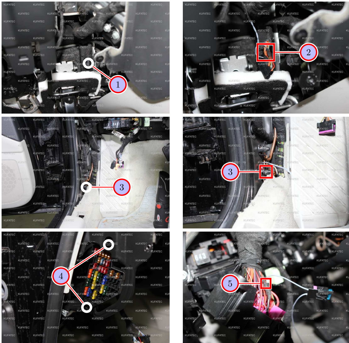
Figure 5: Connection CAN High & CAN Low / ground / ignition lead
