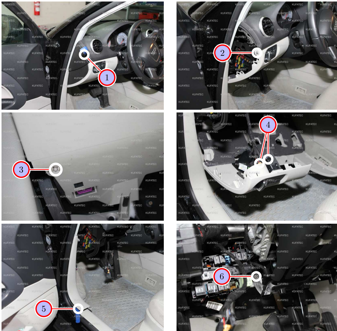
Figure 4: Removing trim panel front driver's side
