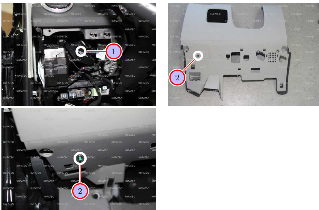
Figure 7: Installation pushbutton
